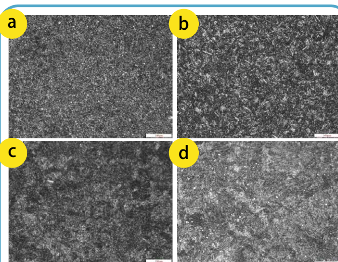
Fig. 5 Metallographic Structure Composed of Lower Bainite, Tempered Troostite, and a Small Amount of Tempered Martensite a. 27MnCrB5 b. 65Mn c. S60C d. SK5
