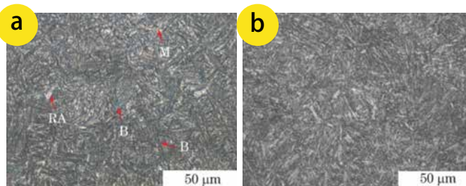
Fig. 4 shows the microstructures of the specimens: 4a shows it is mainly lower bainite + martensite + upper bainite + residual austenite, while 4b shows it is mainly lower bainite + tempered troostite + a small amount of tempered martensite.
