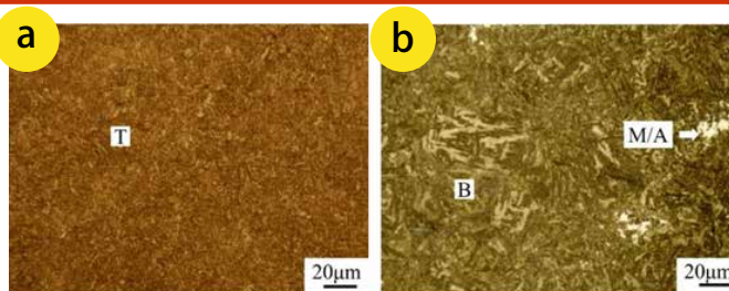
Fig. 3 Microstructure of 51CrV4 Steel by Heat Treatment : (a) Quenching and Tempering Process ; (b) Isothermal Quenching Process
